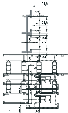
Frame Dimensions 14/18
