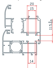
Available profile drawing
