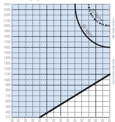
100 kg Load Diagram Glass Weight kg/m
